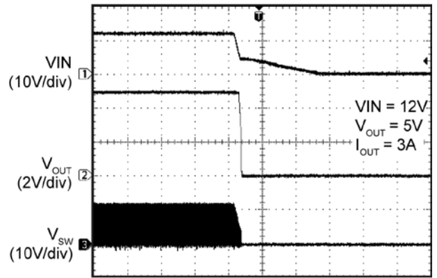
Time (20ms/div)
