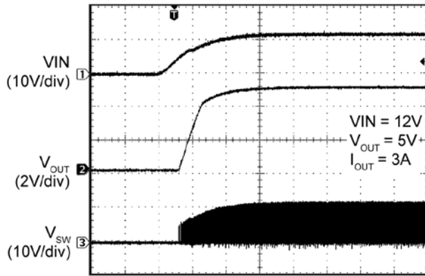
Time (4.0ms/div)
