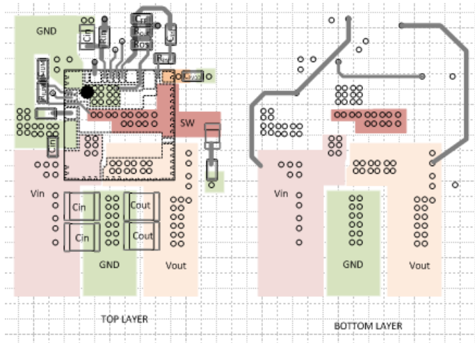
Figure 12. Top And Bottom Layer of a Four-Layer Board
