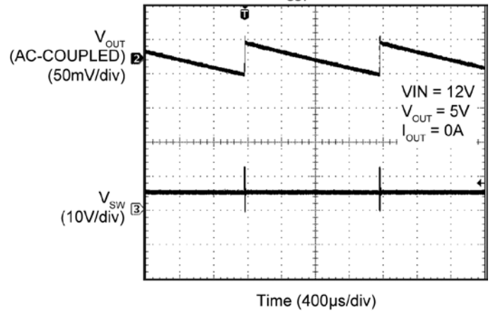
MIC28304-1 Switching Waveforms ( I_{OUT} = 0A )
